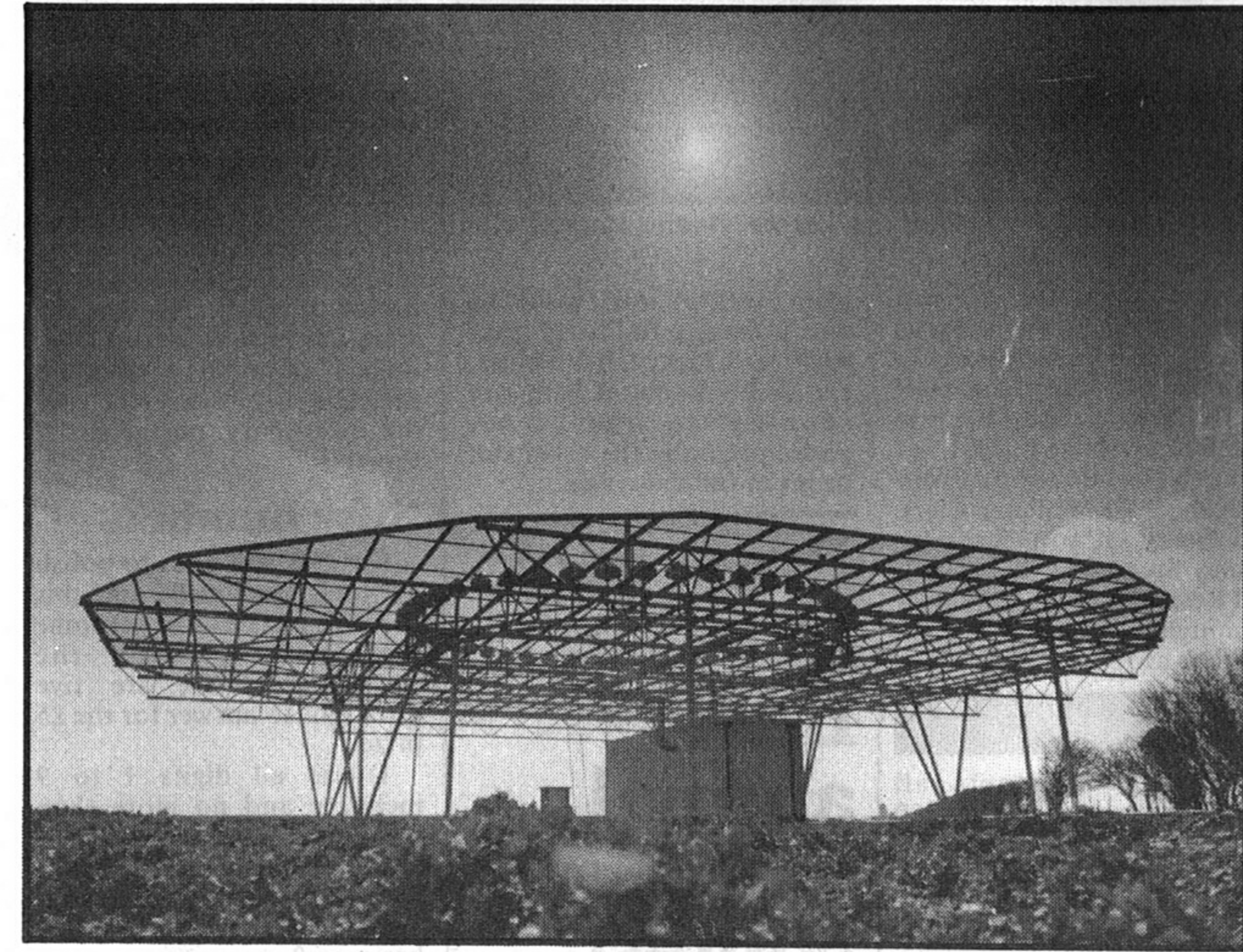
The DVOR installation near St Margarets Bay, Dover.
